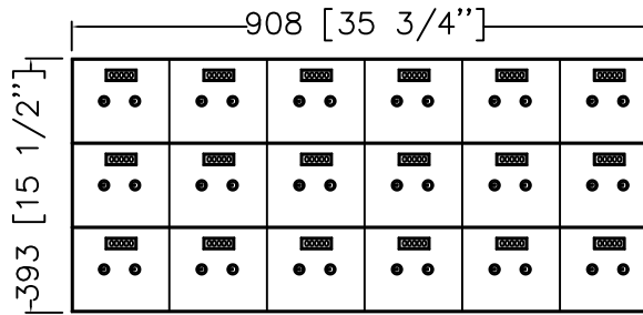
MOLDEL 910 5" x 5" ASSEMBLY 18 OPENINGS.
