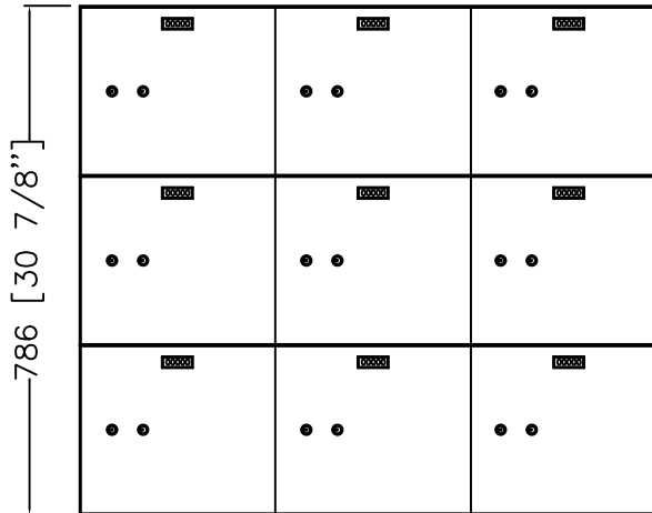
MOLDEL 916 10" x 10" ASSEMBLY 9 OPENINGS.
